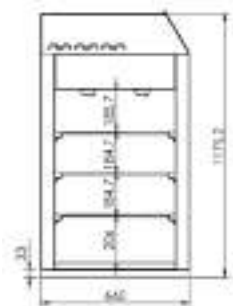
Glass display case without base.
