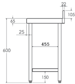
600 series wall-facing table
