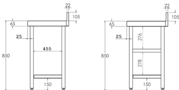
Wall-facing with 1 shelf
