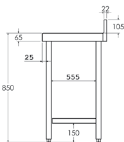
Wall-facing with 1 shelf
