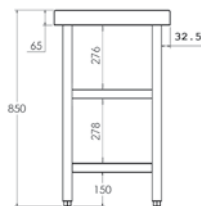
Center with 2 shelves
