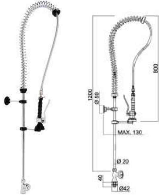
Model Code Single temperature spraying tap • R0020200
