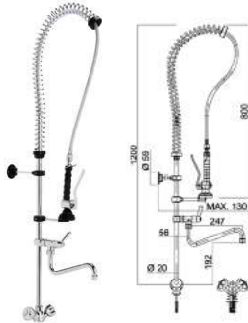
Model Code Spraying tap with hot/cold controls and extra tap • R0020301
