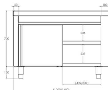
Sliding doors
