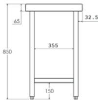
Center with shelf
