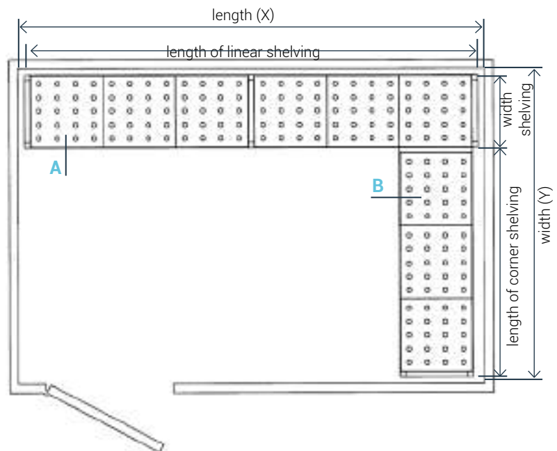
Linear shelving (A)
