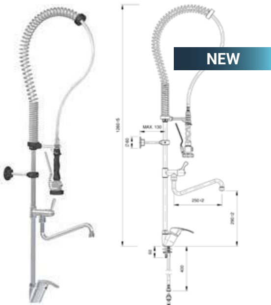
Model Code Single-handle Spraying tap with extra tap • R0020302
