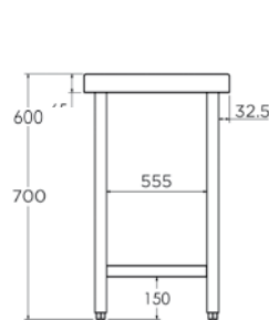
700 series center table
