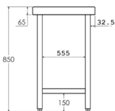
Center with 1 shelf
