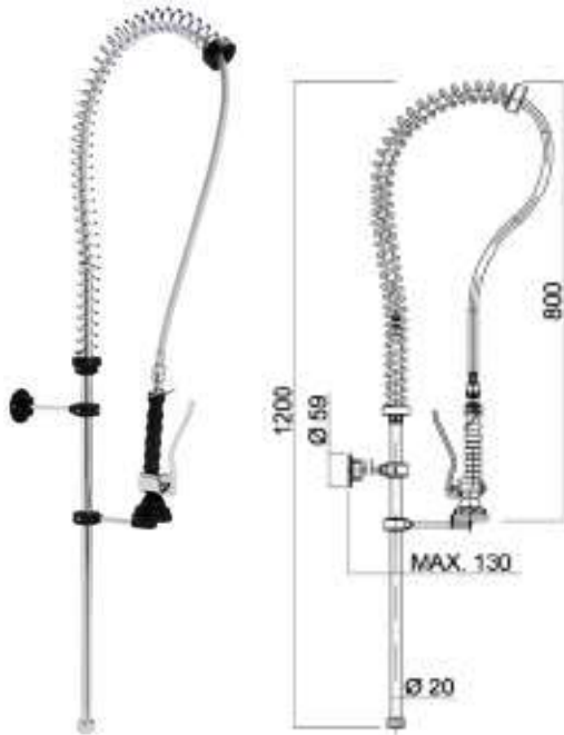
Model Code Spraying tap with no temperature controls • R0020203
