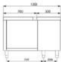
Raised self-service cash register
