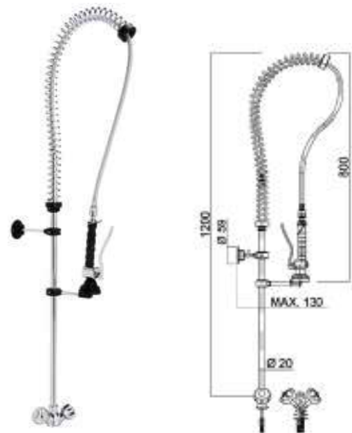
Model Code Spraying tap with hot/cold controls • R0020201
