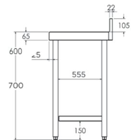
700 series wall-facing table
