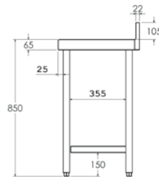
Wall-facing with shelf
