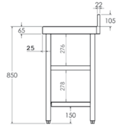
Wall-facing with 2 shelves
