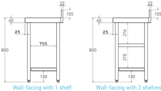
Wall-facing with 1 shelf
